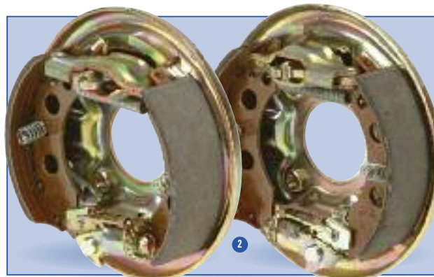
2 P00130 Complete 2051 brake assembly (axle set). Pre-fitted to backplate and complete with all springs, adjusters etc. Fitted from Jan 1989 – September 1992. £140.00
