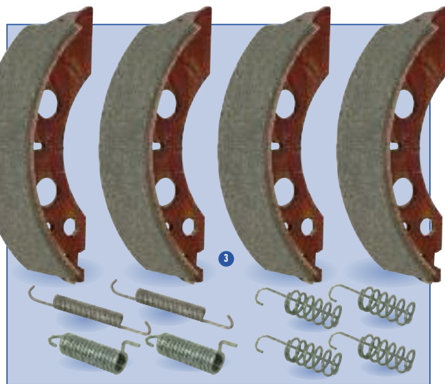
3 P00860 Brake shoe set. 2051 brake (will also fit 2050 brake). £59.00 A full set comprising of four brake shoes and all springs required to complete the installation. This kit services one axle, for continued safety, brakes should always be changed as complete axle sets.
